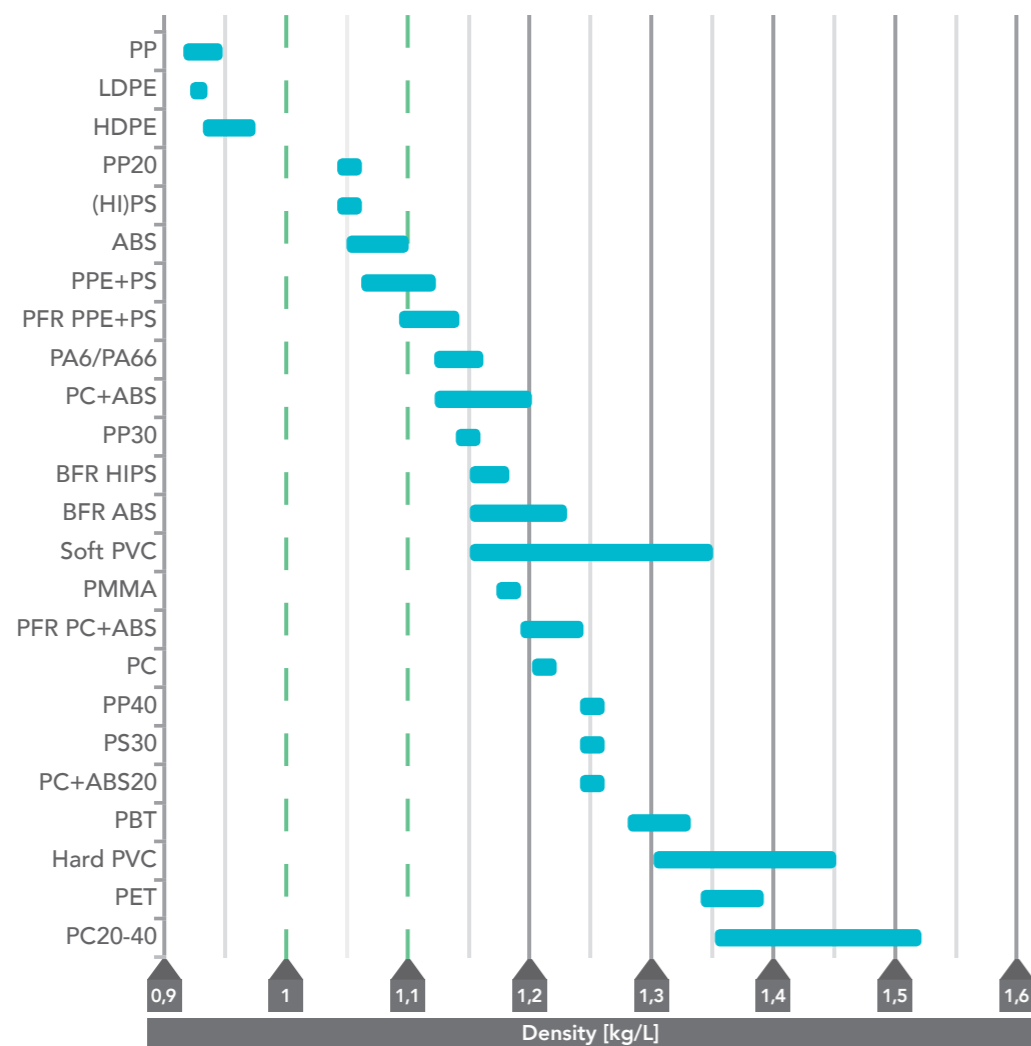
Figure 11 : Density range of common WEEE plastics 16,31-33 . PFR = organophosphorus flame retardants. BFR = brominated flame retardants. PP20/30/40/50 = PP filled with 20/30/40/50% glass-fiber, talc or other mineral fillers. PS30 = PS filled with 30% glass-fiber. PC20-40 = PC with 20-40% glass-fiber. PC-ABS20 = PC-ABS filled with 20% glass-fiber
