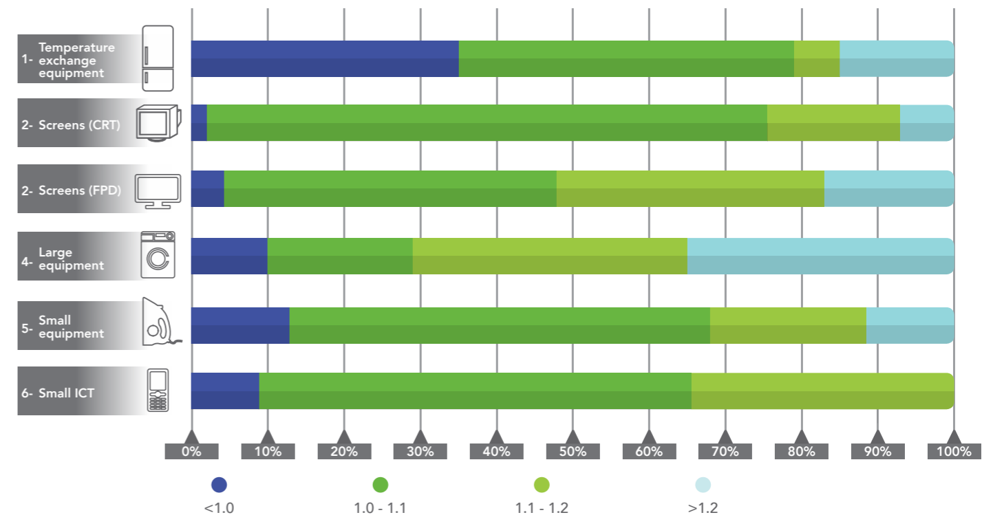
Figure 14: Densimetric profile of WEEE plastics (in kg/L)
