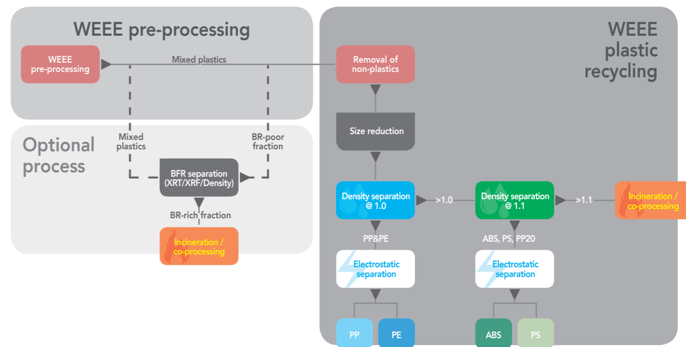
Figure 12 : Conventional WEEE plastic treatment processes
