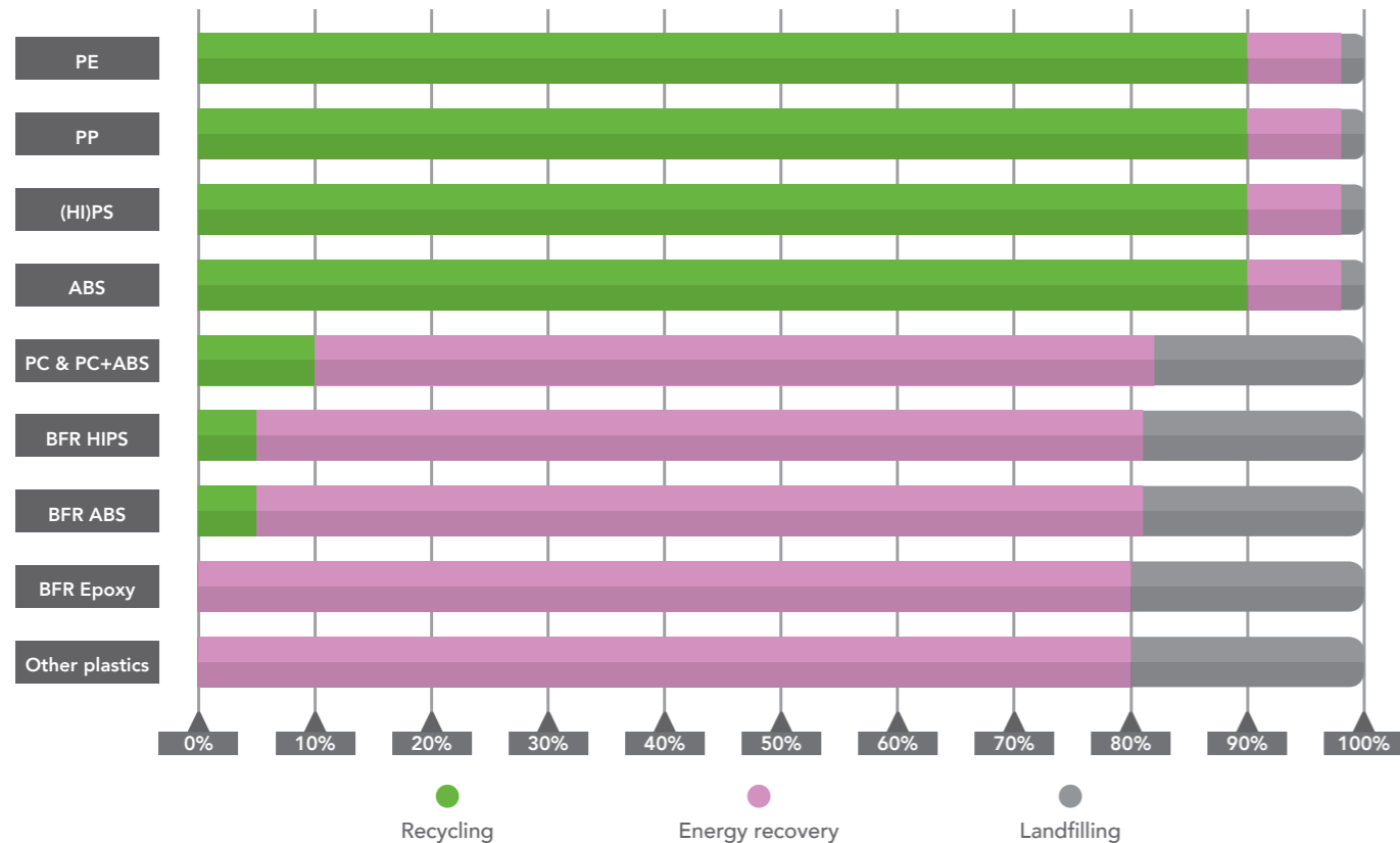
Figure 6: Output of WEEE plastics recycling, by plastic type. In the case of BFR Epoxy, energy recovery mainly refers to treatment of printed circuit boards in copper smelters, whereby the epoxy acts as fuel substitute (and reducing agent).
